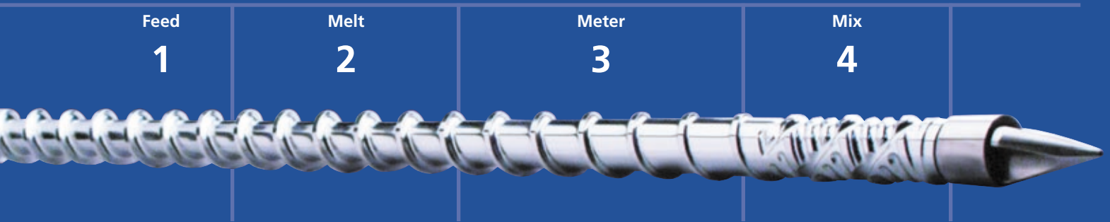
The Xaloy StrataMelt™ Injection Screw
